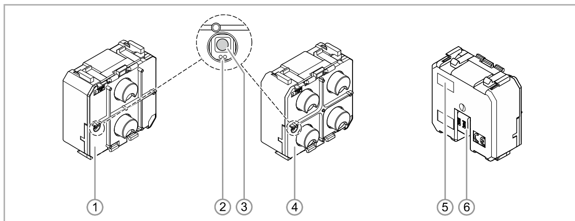
Fig. 2: Overview of devices of push-button coupling units
